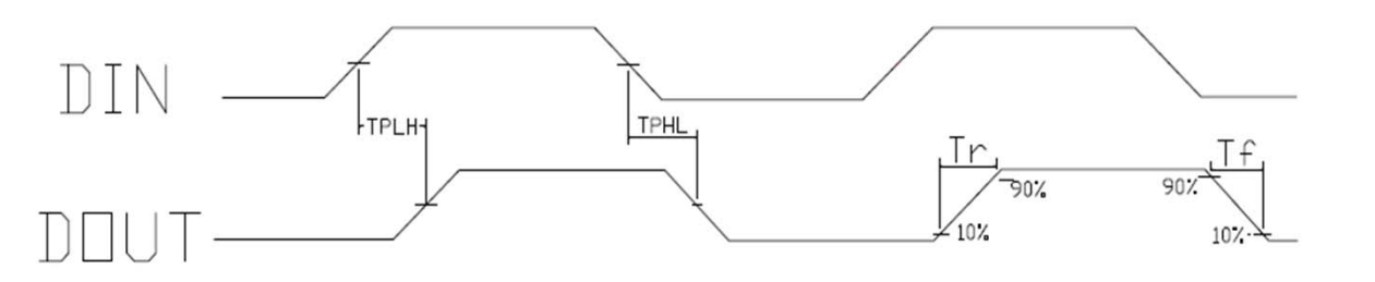
10. The data transmission time (TH+TL=1.25μs±600ns):
